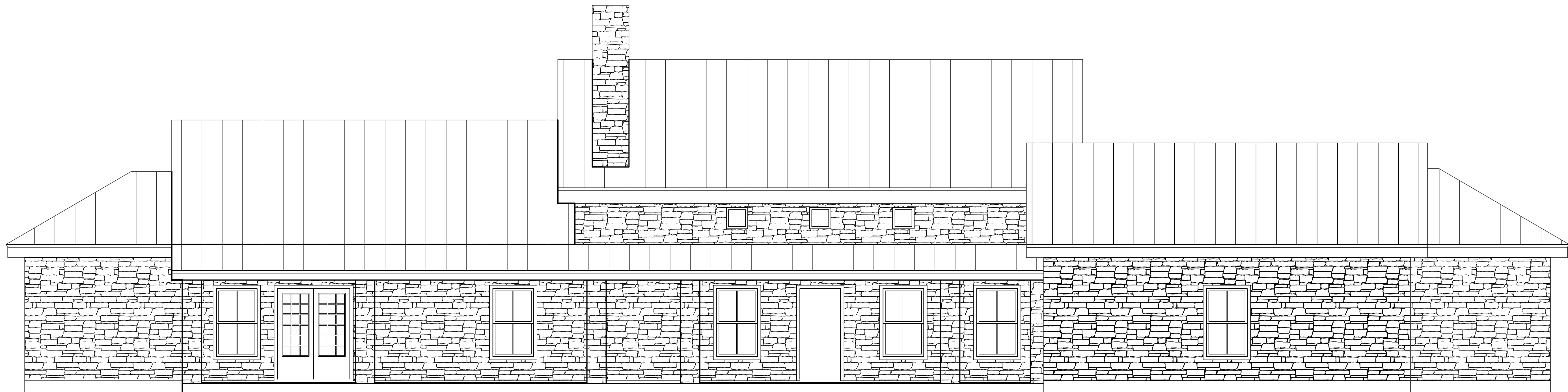
A FRONT ELEVATION
